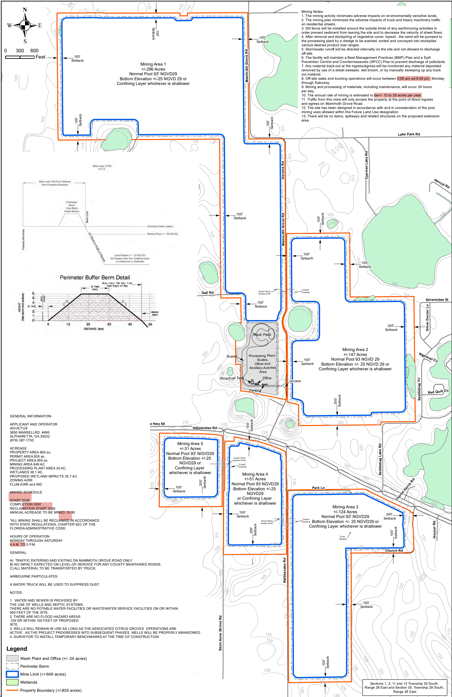
Figure 9 Mine Plan Mammoth Grove Mine Mammoth Grove Road Lake Wales, Polk County, Florida
