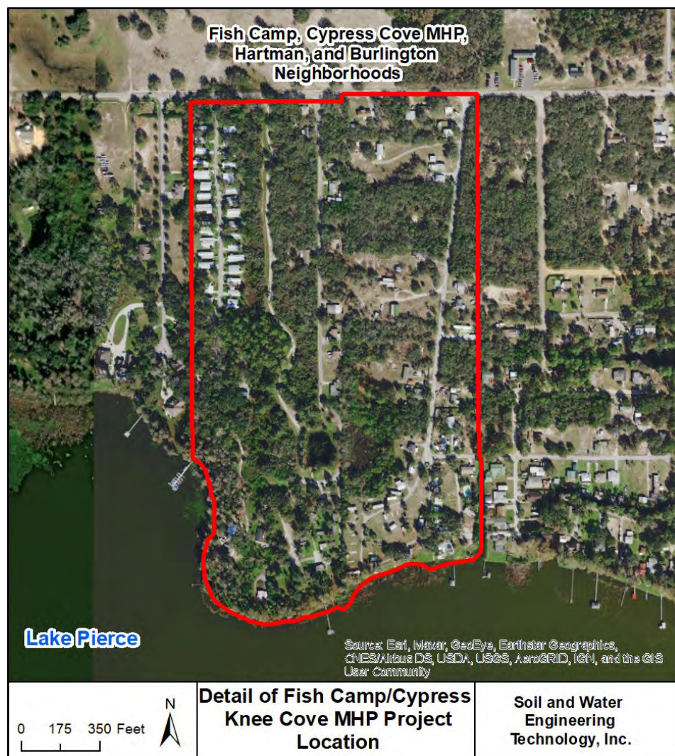
Figure 4. Detail of Area 1: location of the Jennings Resort and FCHB project areas.
