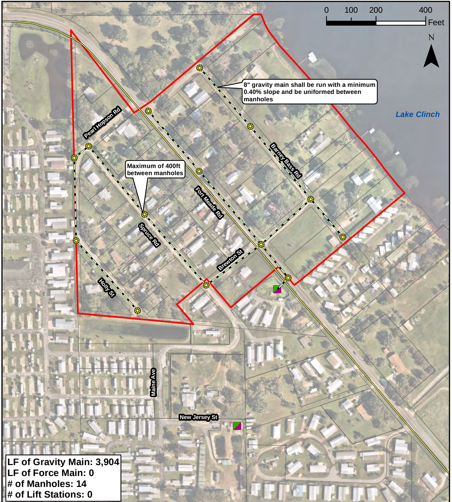
FIGURE 4 Polk County Utilities Septic to Sewer Preliminary Layout Bay View Park Subdivision
