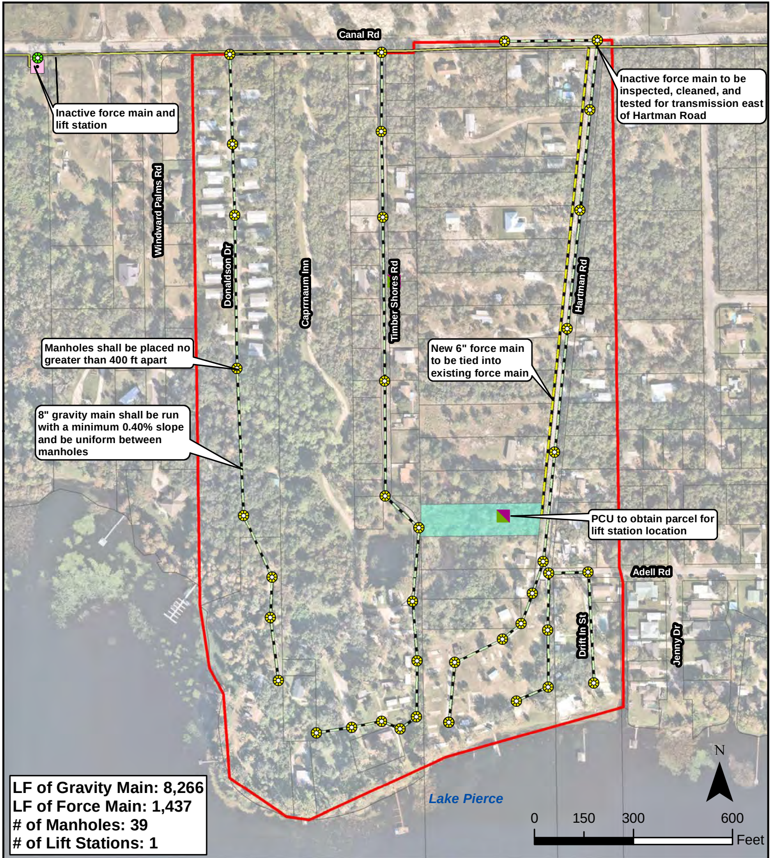
FIGURE 5 Polk County Utilities Septic to Sewer Preliminary Layout Timber Shores, Cypress Knee Cove MHP, Burlington and Hartmans Neighborhoods
