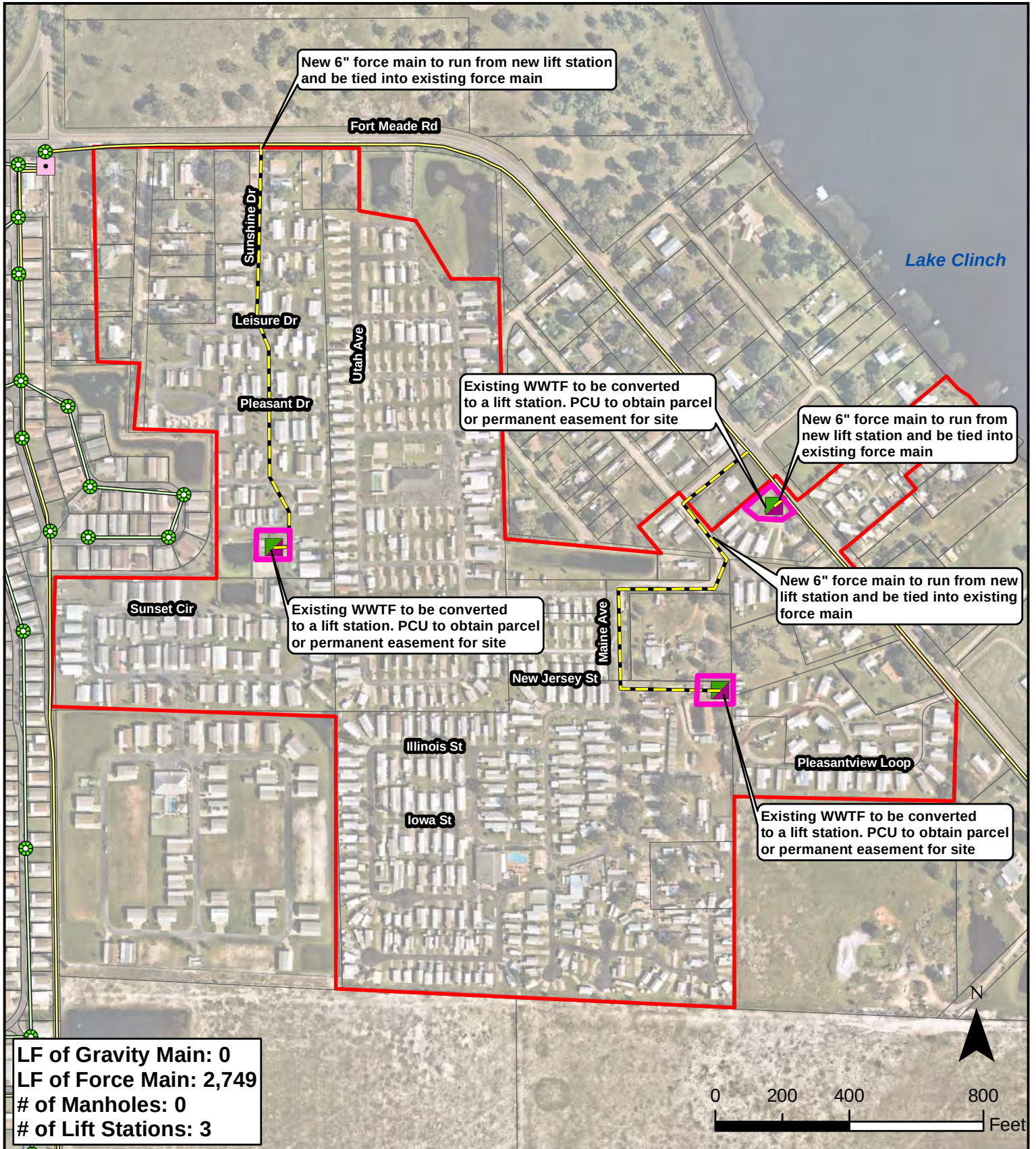
FIGURE 2 Polk County Utilities Septic to Sewer Preliminary Layout Whispering Pines MHP & Lakemont Ridge Home and RV Park
