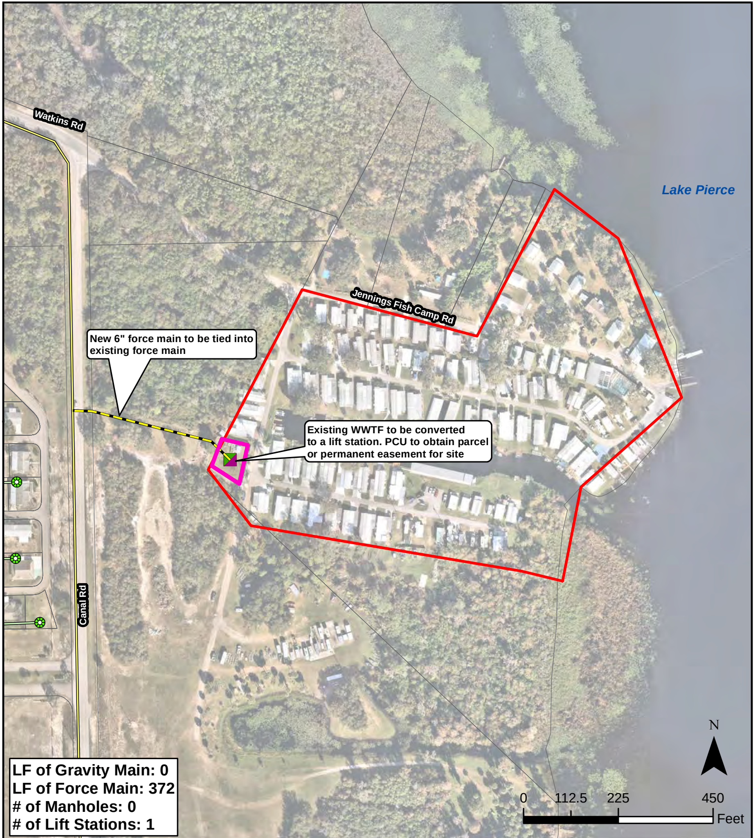
FIGURE 1 Polk County Utilities Septic to Sewer Preliminary Layout Jennings Resort Mobile Home Park
