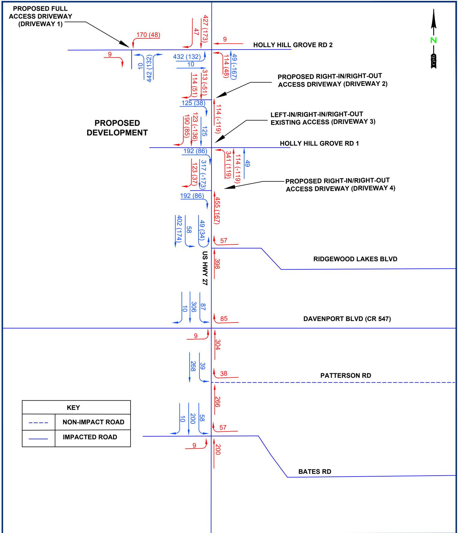
FIGURE 6B - TRAFFIC ASSIGNMENT P.M. RETAIL WITH OUTPARCELS DAVENPORT, POLK COUNTY, FLORIDA
