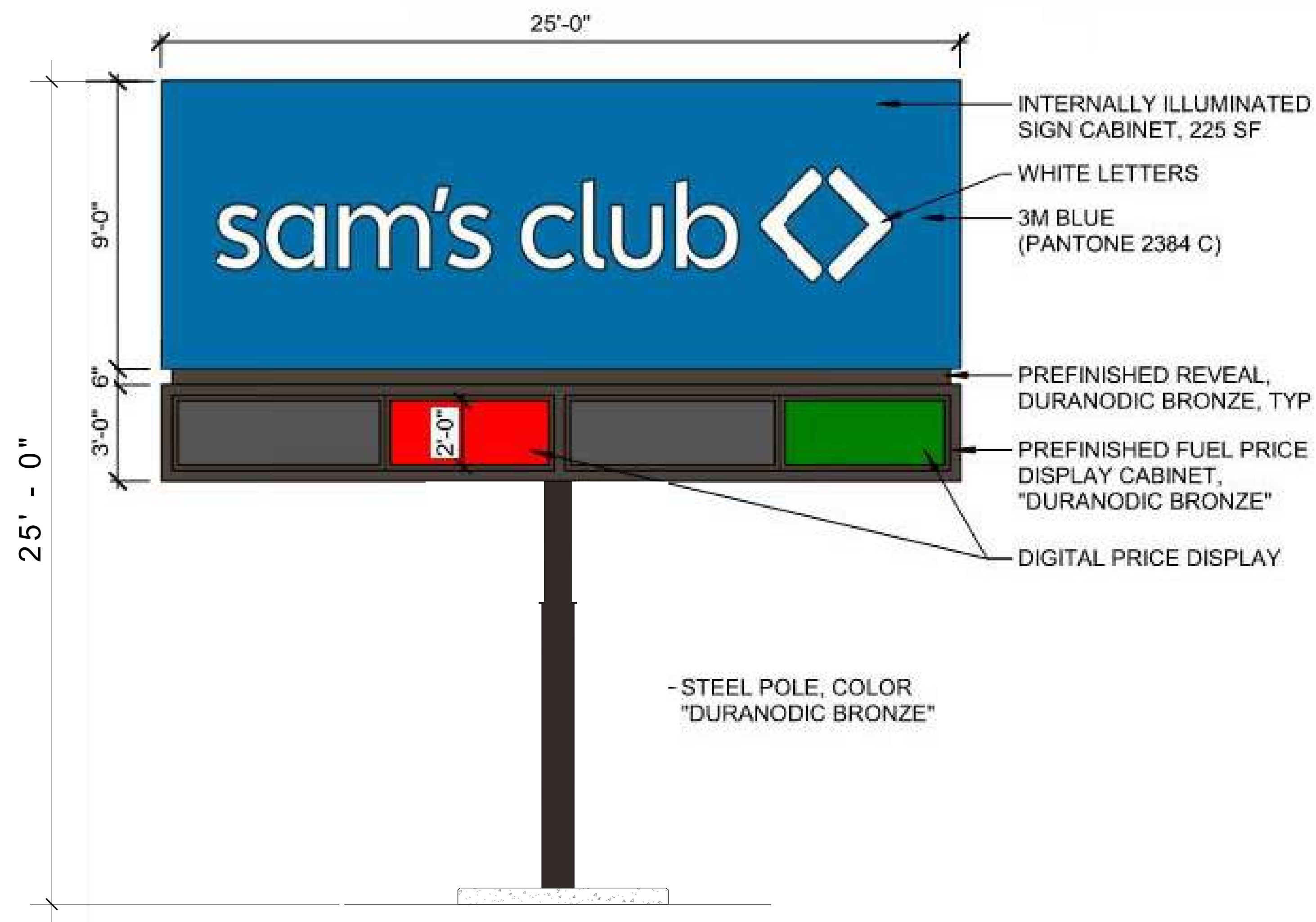
2 25'-0" PYLON SIGN 3/8" = 1'-0"
