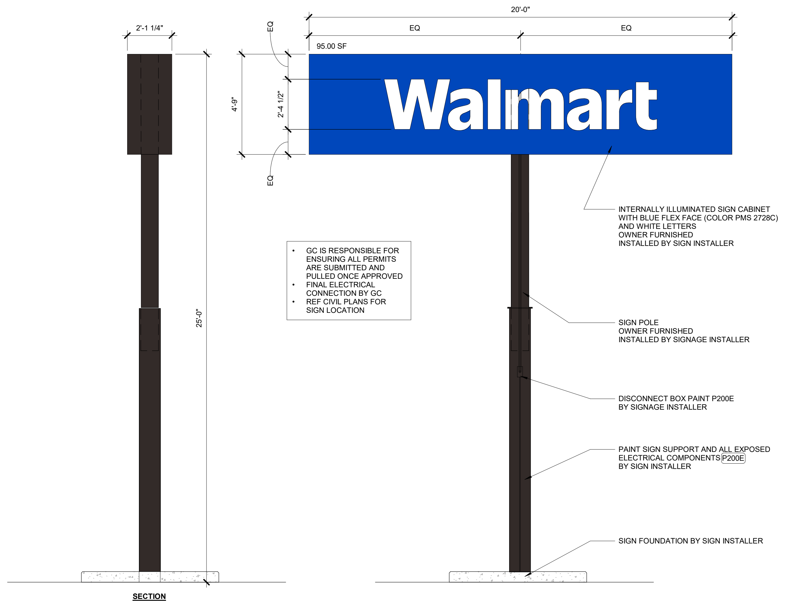
1 25'-0" PYLON SIGN 3/8" = 1'-0"
