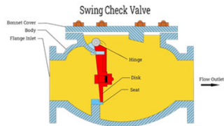
Check Valves required in low areas
