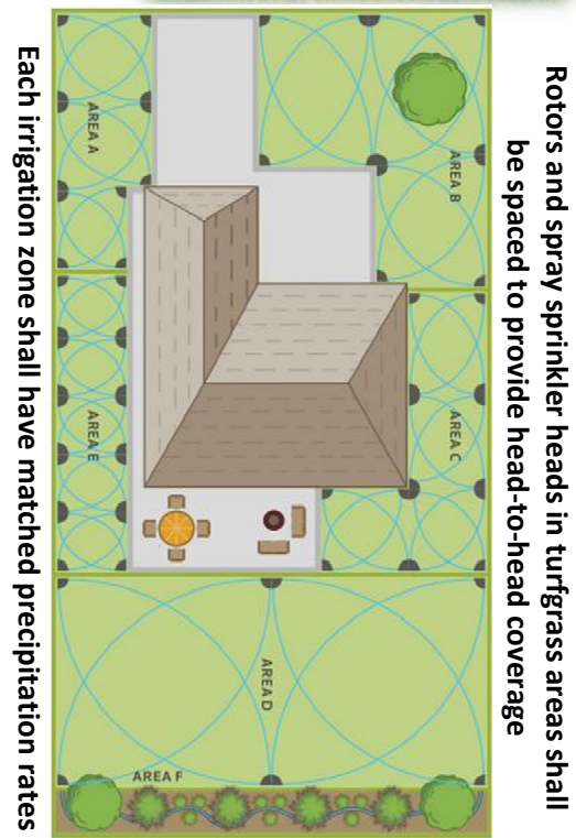
Sprinkler head types, such as spray heads and rotors, shall not be mixed in the same zone
