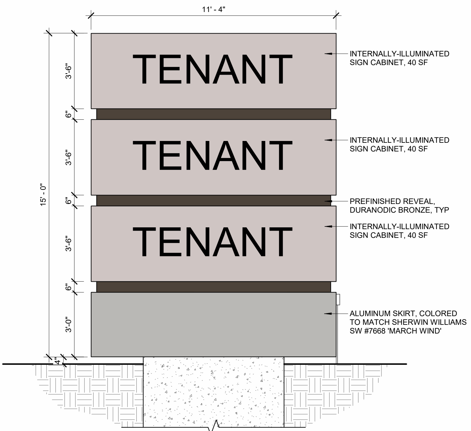
2 Monument Sign B 3/8" = 1'-0"
