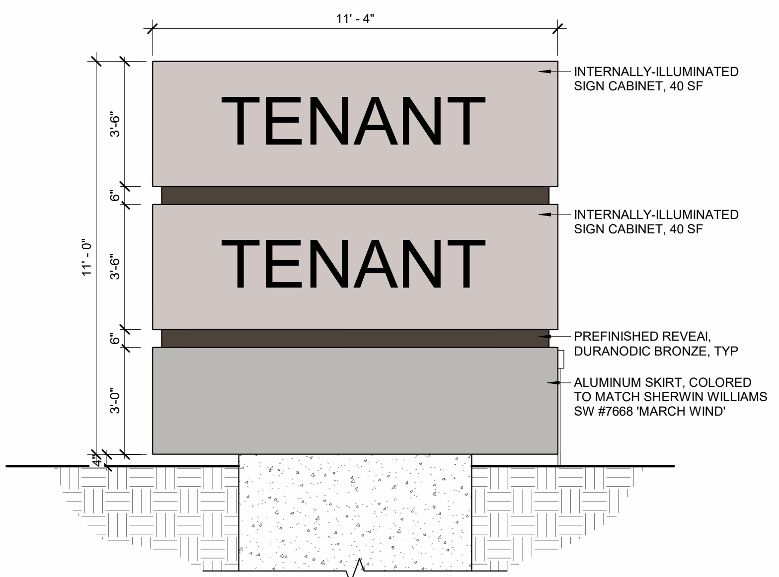
3 Monument Sign C 3/8" = 1'-0"
