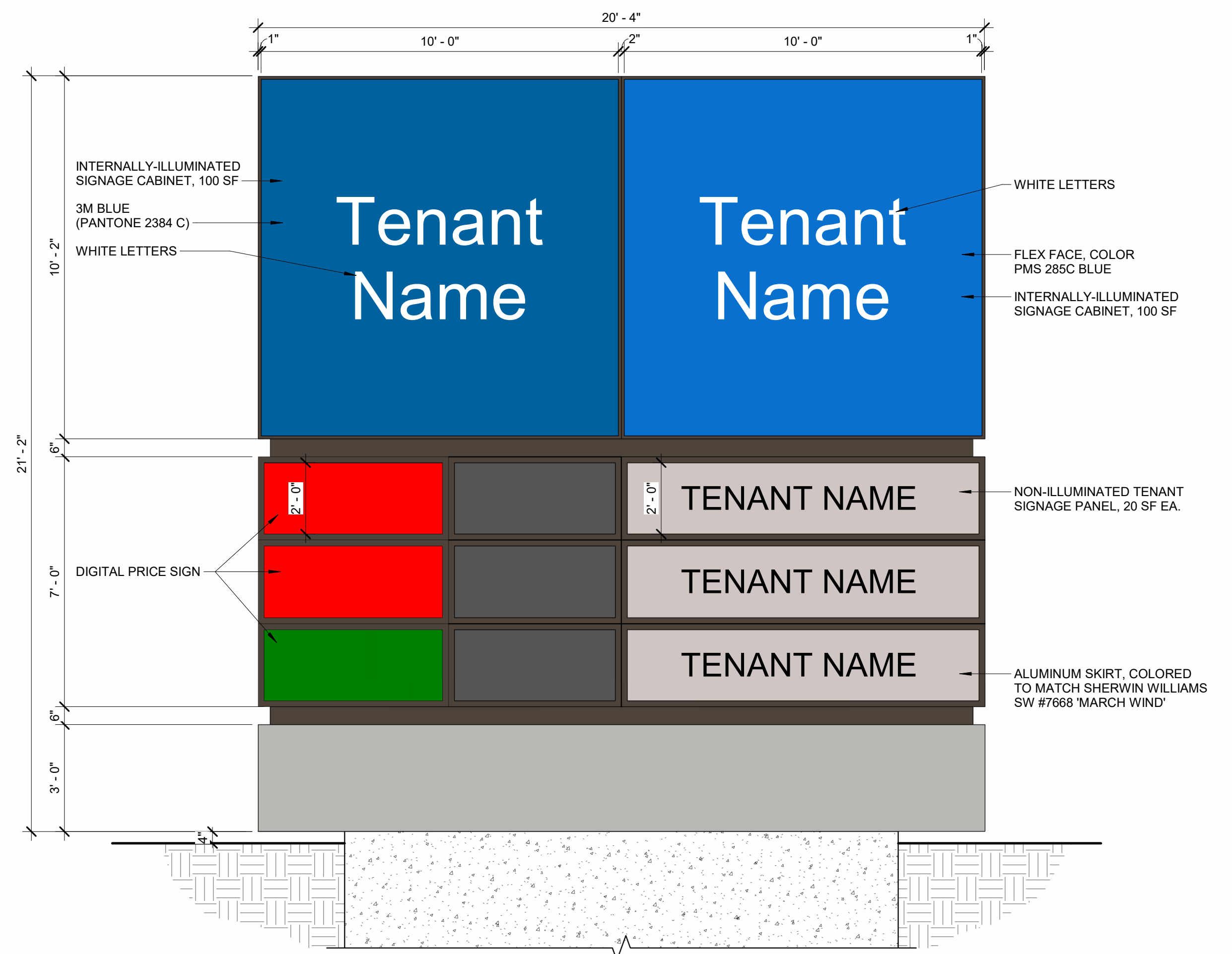
1 Plaza Sign A 3/8" = 1'-0"
