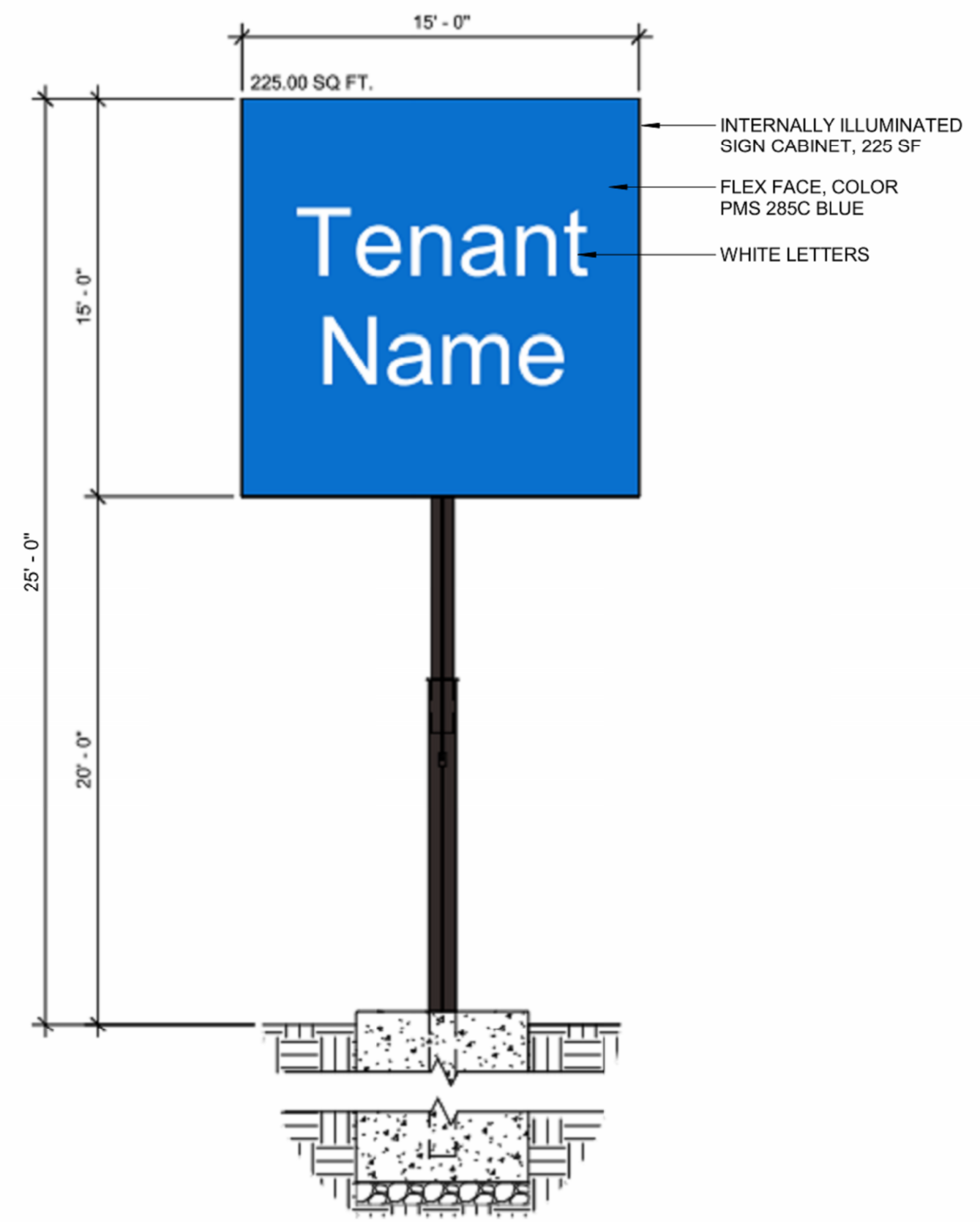
4 Pylon Sign D 3/16" = 1'-0"
