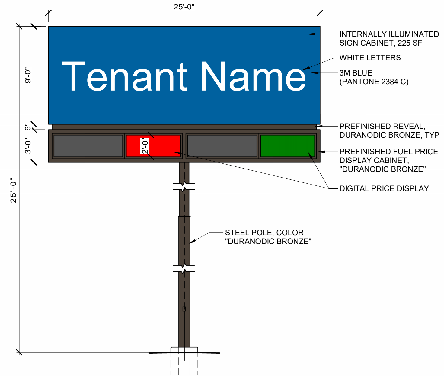
5 Pylon Sign E 3/16" = 1'-0"
