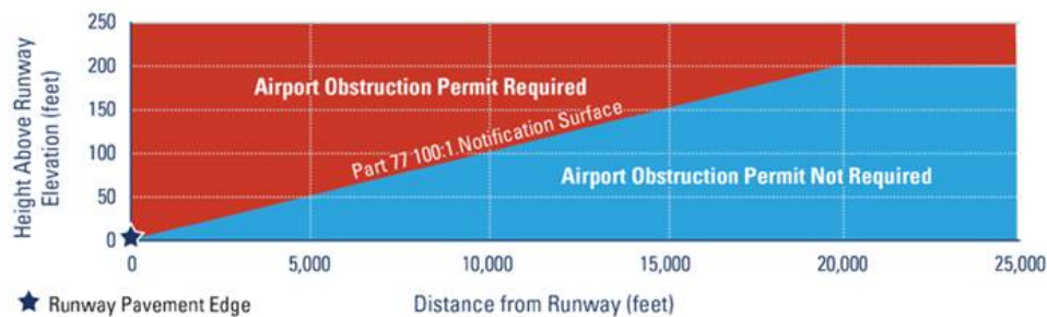
Figure 10. 14 CFR Part 77.9 Notification Surfaces for Airports Where the Longest Runway is More than 3,200 Feet
